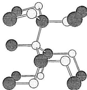
Figure 1: The orthorhombic supercell of wurtzite CdS. Smaller spheres describe anions (S) and larger cations (Cd). The upper half of the supercell illustrates the relaxed (10 \bar{1} 0) surface but the lower half is fixed to the bulk geometry. There are eight inequivalent atoms (two primitive cells) in the corresponding bulk supercell (6.72 Å \times 4.14 Å \times 7.17 Å) and ten atoms in the supercell of the thinnest slab model.
