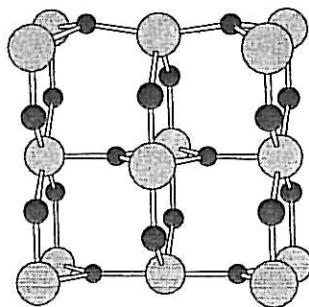
Figure 2: The orthorhombic supercell of rutile \text{SnO}_2 . Smaller spheres describe anions (O) and larger cations (Sn). The upper half of the supercell illustrates the relaxed (110) surface but the lower half is fixed to the bulk geometry. There are 12 inequivalent atoms (two primitive cells) in the corresponding bulk supercell ( 6.67 \text{ \AA} \times 3.19 \text{ \AA} \times 6.67 \text{ \AA} ) and 15 atoms in the supercell of the thinnest slab model.
