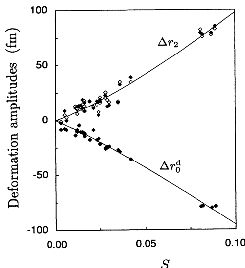
FIG. 5. The dependencies of the deformation amplitudes \Delta r_0^d and \Delta r_2 on the order parameter S . The points are calculated by Eqs. (3) and (4) (◇) as well as (5) and (6) (◆) from the results of all the simulations (Monte Carlo and molecular-dynamics runs in the square and hexagonal lattice, including the special simulations with the modified potentials). The solid lines are least-squares fits to the data (including the points at S = 0.25 , which are not shown in the figure) using the polynomials c_1 S + c_2 S^2 + c_3 S^3 . The values of the coefficients c_1 , c_2 , and c_3 are -732 , -3207 , and 9716 fm (for \Delta r_0^d ) and 604 , 5198 , and -14\,464 fm (for \Delta r_2 ).
