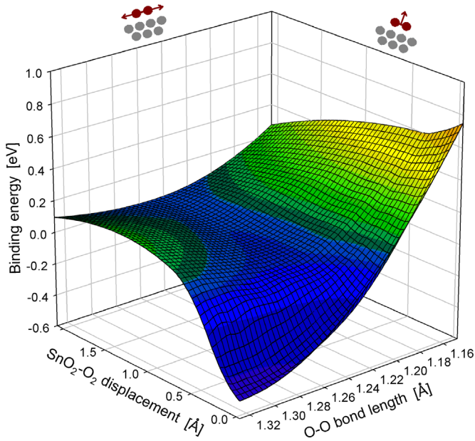
Fig. 3. The calculated potential-energy surface representing the binding energy of oxygen molecule adsorbed at the \text{SnO}_2 \text{Sn}_{5c} through as a biaxial function of O–O bond length and displacement of \text{O}_2^- center of mass from its optimized position, induced by vibration modes.
