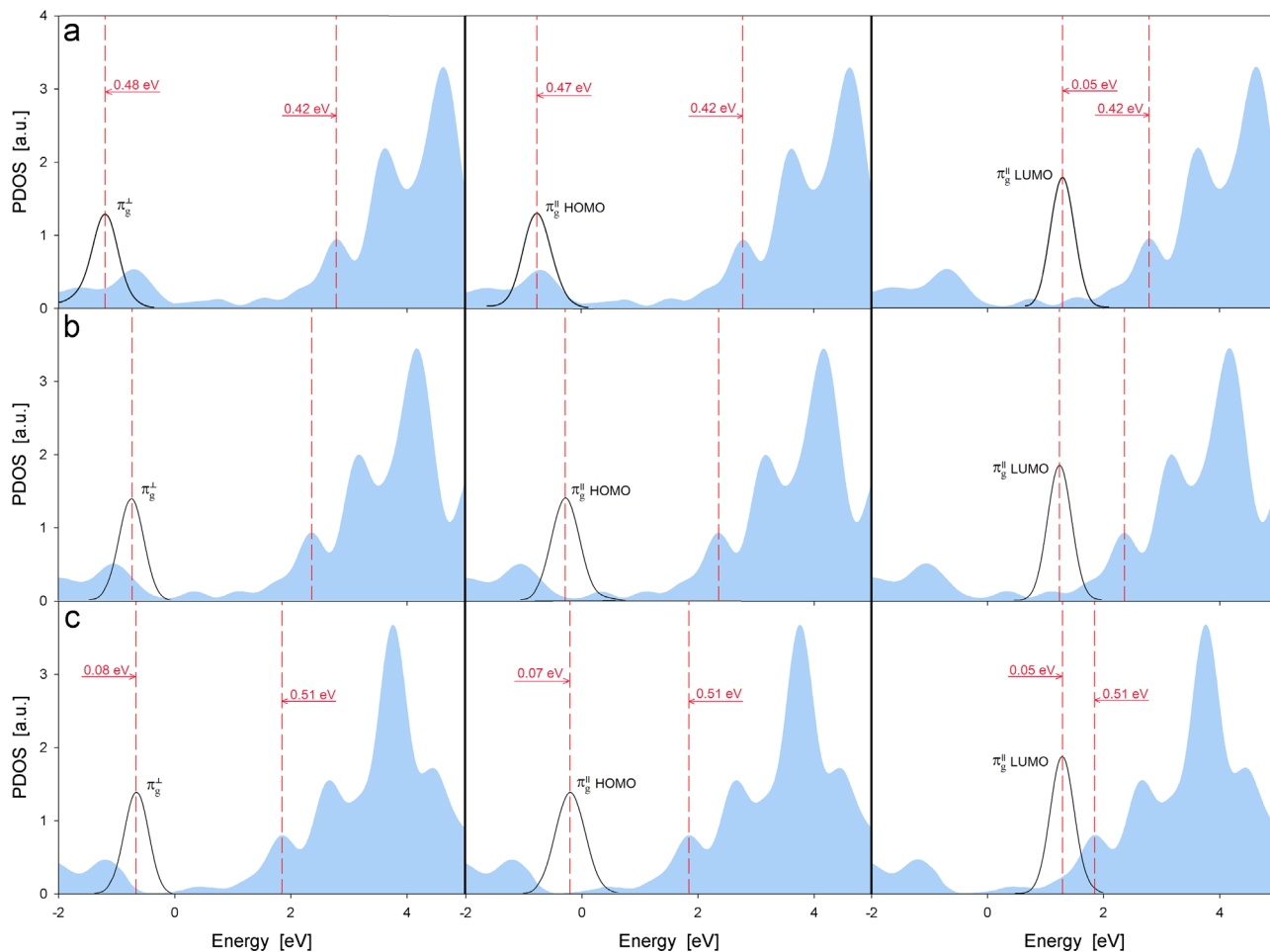
Fig. 4. The PDOS of the Sn_{5c} surface atoms (blue area) and the PDOS of the \pi_g^\perp hybrid orbital (left panel); the \pi_g^\parallel HOMO (center panel) and the \pi_g^\parallel LUMO (right panel) of the O_2^- molecule adsorbed on-top of the Sn_{5c} surface atoms (black line) calculated for (a) compressed by 2% surface, (b) surface with equilibrium lattice constants, and (c) surface stretched by 2%. The red arrows indicate direction and values of the shifts in the energetic position of the corresponding orbitals. (For interpretation of the references to color in this figure legend, the reader is referred to the web version of this article)
