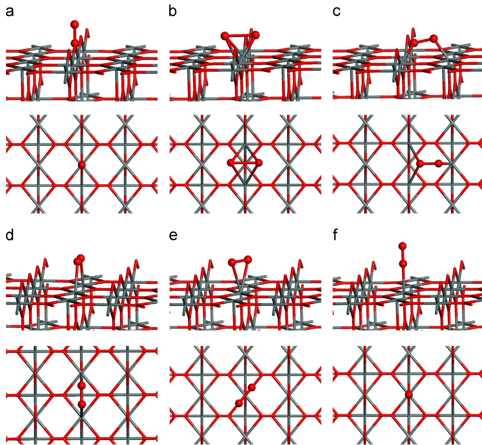
Fig. 1. The side and top views of the molecular oxygen adsorption structures adsorbed at SnO 2 (110) surface. Sn and O atoms of the slab are represented as gray and red sticks, respectively, while adsorbed O atoms are represented as red spheres. (For interpretation of the references to color in this figure legend, the reader is referred to the web version of this article)
