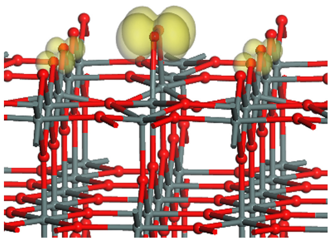
Fig. 2. Isosurface of spin density distribution (contoured at 0.05\text{e}^{-}\text{\AA}^{-3} ) for superoxide \text{O}_2^- molecule adsorbed at \text{Sn}_{5c} trough.
