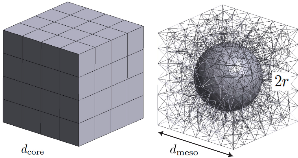
Fig. 2. Left: the homogenized macro-scale CM domain of the original problem. Right: the meso-scale cell representing the CM.
