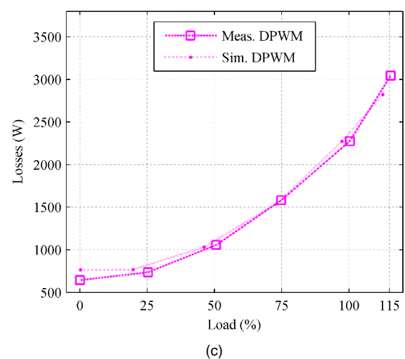
Fig. 6. Comparison of the measured and simulated total electromagnetic losses with (a) DTC, (b) PWM and (c) DPWM supplies. The measured total electromagnetic losses is obtained by subtracting the mechanical output power and the friction and windage losses of 152 W from the electric input power.
