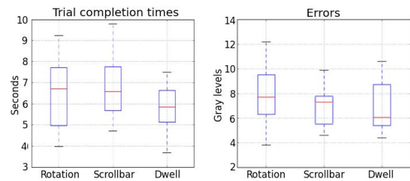
Figure 2. Task completion times (left) and errors (right). Note that in this boxplot the line in the middle shows the median.
